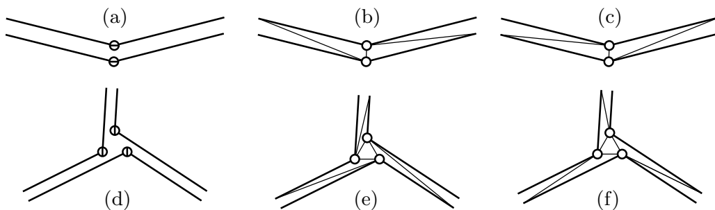
Fig. 2 A wire (a) that transfers TRUE (b), and FALSE (c), and a variable (d) in TRUE (e) and FALSE (f) state. The short edges are part of in every triangulation.
