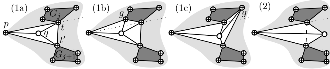
Fig. 6 Construction for the lower bound using the order type data base results. The gray regions depict the convex hulls of groups of eleven points. The three different cases to handle the separating vertices are shown.
