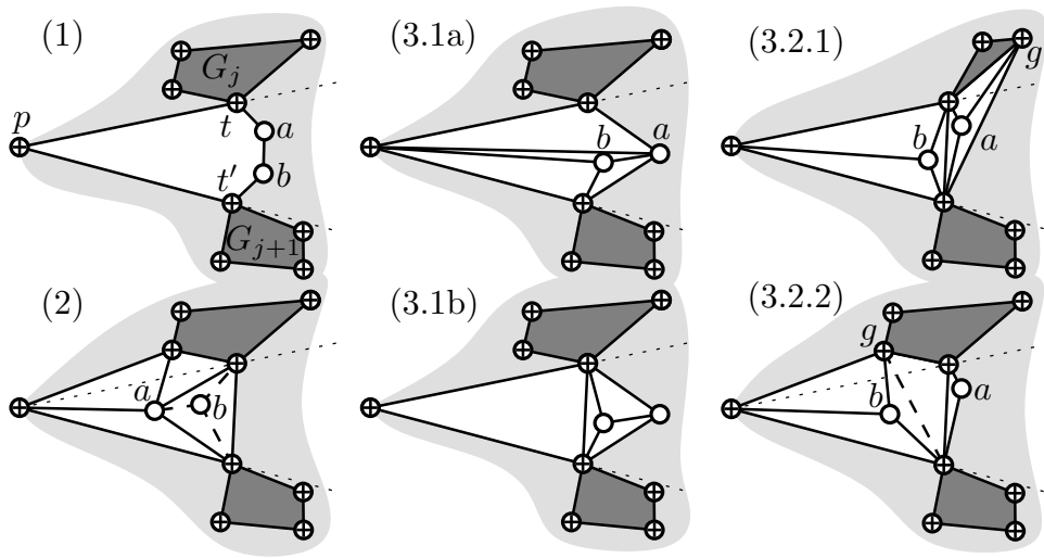
Fig. 7 Two vertices between two groups can be made odd. Examples for the different cases are shown, as well as the two possibilities for Case (3.1). The dashed stroke for Case (3.2.2) depicts the flipped edge.
