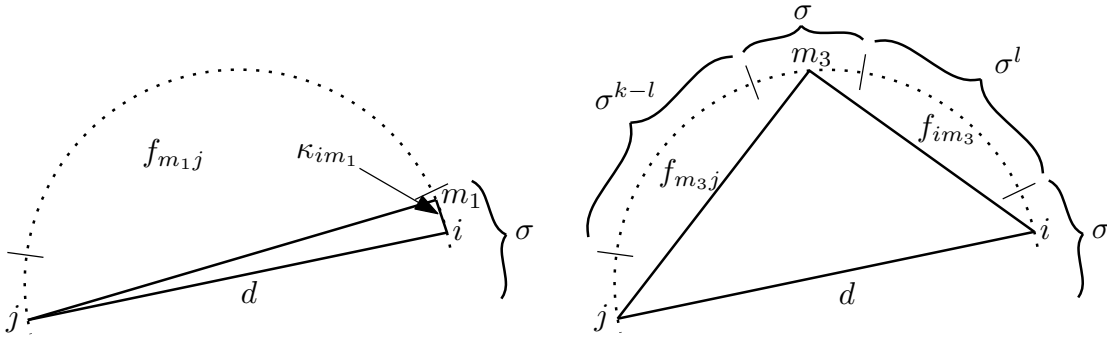
Fig. 5 The different types of subproblems formed by triangles with their base at d .
