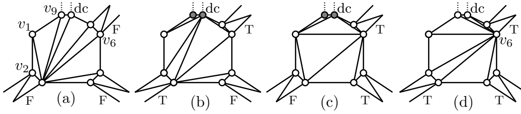
Fig. 4 An OR-gate with inputs FALSE, FALSE (a), TRUE, FALSE (b), FALSE, TRUE (c), and TRUE, TRUE (d). The two inputs are at the bottom and the output is at the upper right side. A don't-care loop “dc” is attached to the two top-most vertices.
