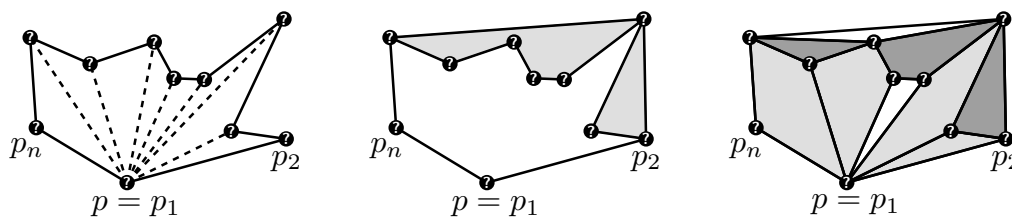
Fig. 8 The simple polygon bounded by P , the initial graph T_0 (with dark faces shown gray), and the graph T_1 in which all faces are convex (interesting light and dark faces shown light gray and dark gray, respectively).
